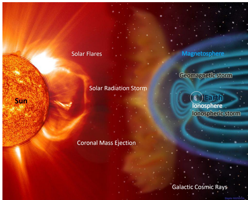
Figure 1. Space weather phenomena, adapted from https://picryl.com/media/space-science-12eac1
