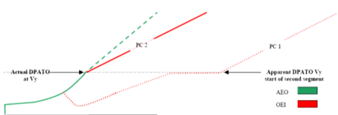
Figure 9: Using Cat A data; actual and apparent position of DPATO ( V_y and start of second segment)
