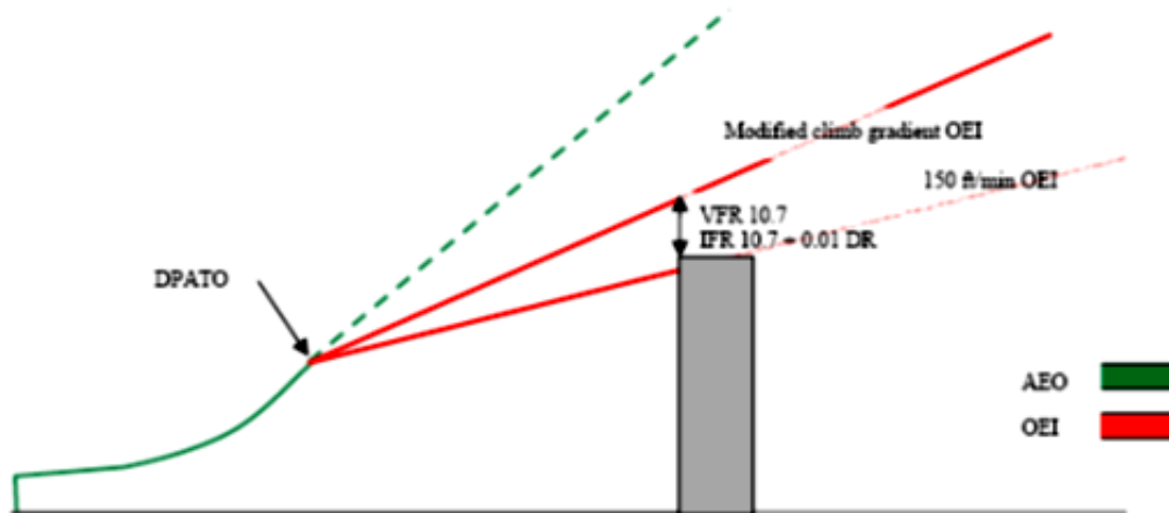
Figure 6: Performance Class 2 (enhanced climb gradient)
