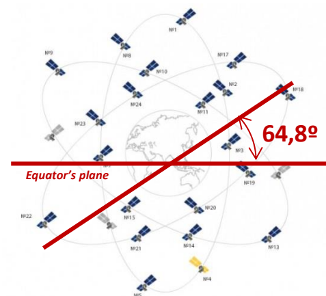
GLONASS Constellation (Source: http://www.spacecorp.ru/en/directions/glonass/orbital/ )
